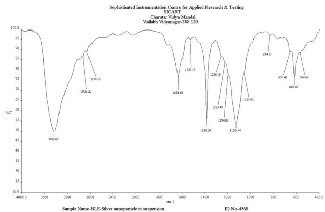
Figure 5: FTIR spectrum of silver nanoparticles synthesized by using the leaf extract of Bambusa arundinaceae .
