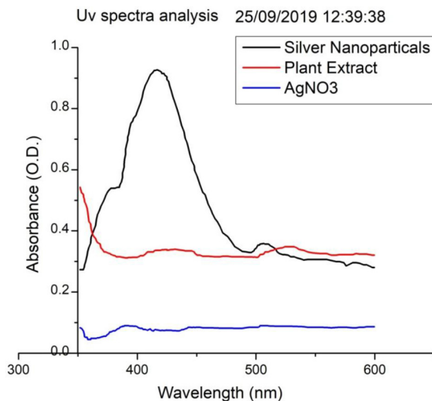
Figure 3: UV-VIS spectroscopy for silver nanoparticles (BA-AgNPs), \text{AgNO}_3 solution and leaf extract of Bambusa arundinaceae .
