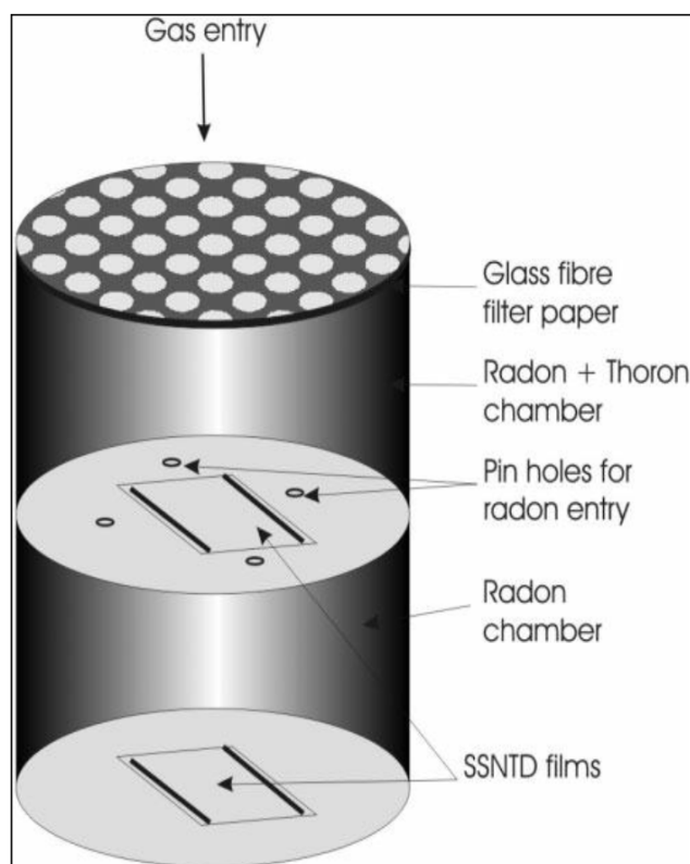
Figure 2: Schematic diagram of Single-entry Pin-hole dosimeter. [8]
