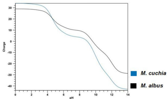
Figure 4c. Electrical vs pH graph for Glutathione S-transferase in M. cuchia and M. albus .
