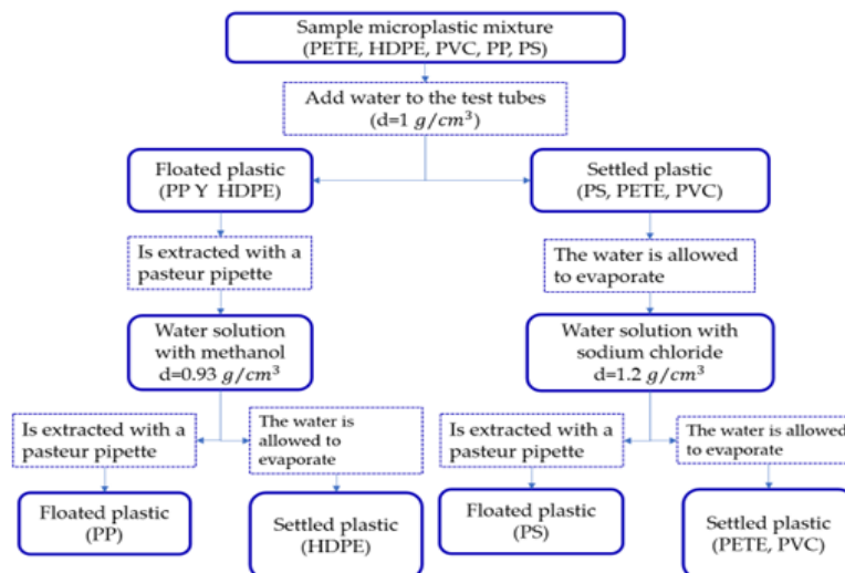
Figure 2: Separation diagram of MPs, by difference in densities (Own).
