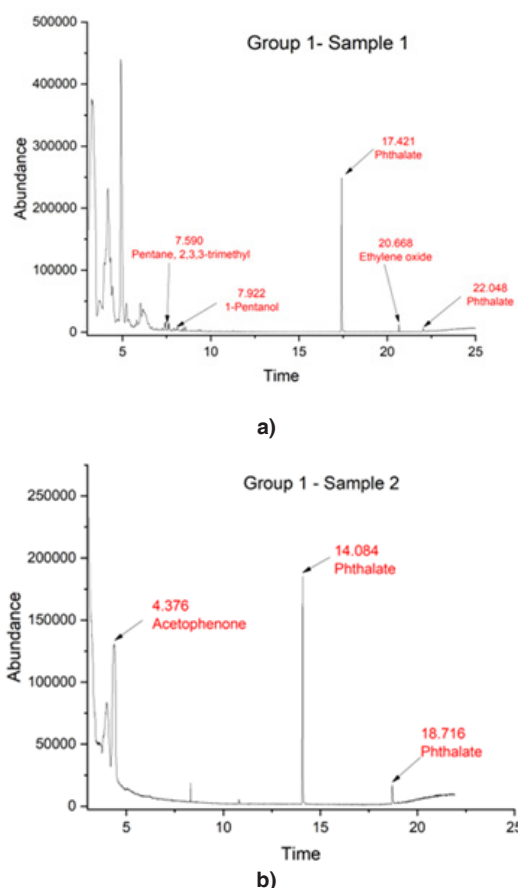
Figure 8: Example of chromatogram obtained from: a) sample 1; b) sample 2. (Own work)
