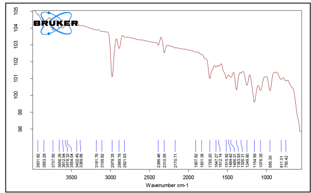
Figure 6: ATR-FTIR Spectrum of microsponge formulation.
