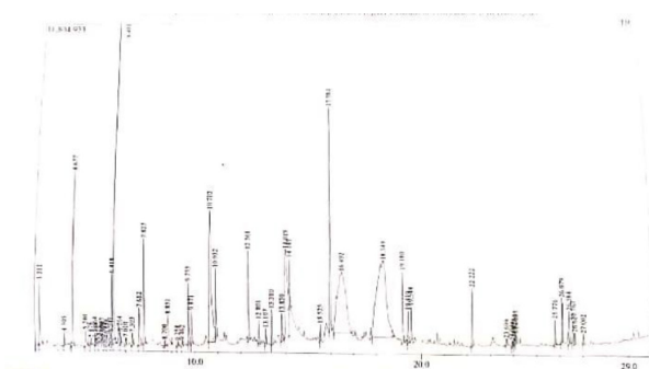
Figure 1: GC/MS Chromatogram Spectrum of M. longifolia oil extract.
